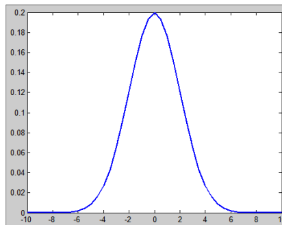
Figure 3.4: A Gaussian kernel with mean = 0 and standard deviation = \sqrt{2}
